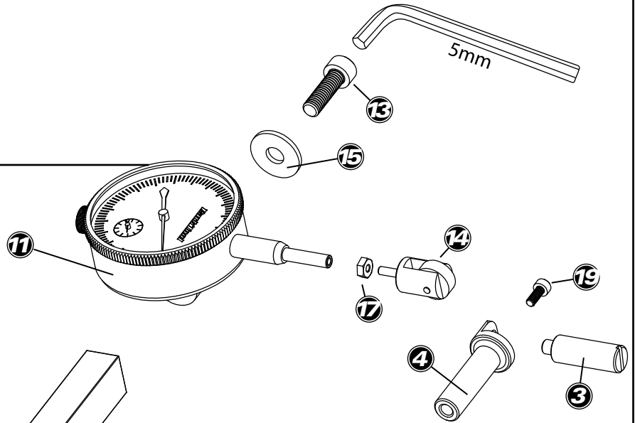
Figure 2 Radial Dial Assembly
